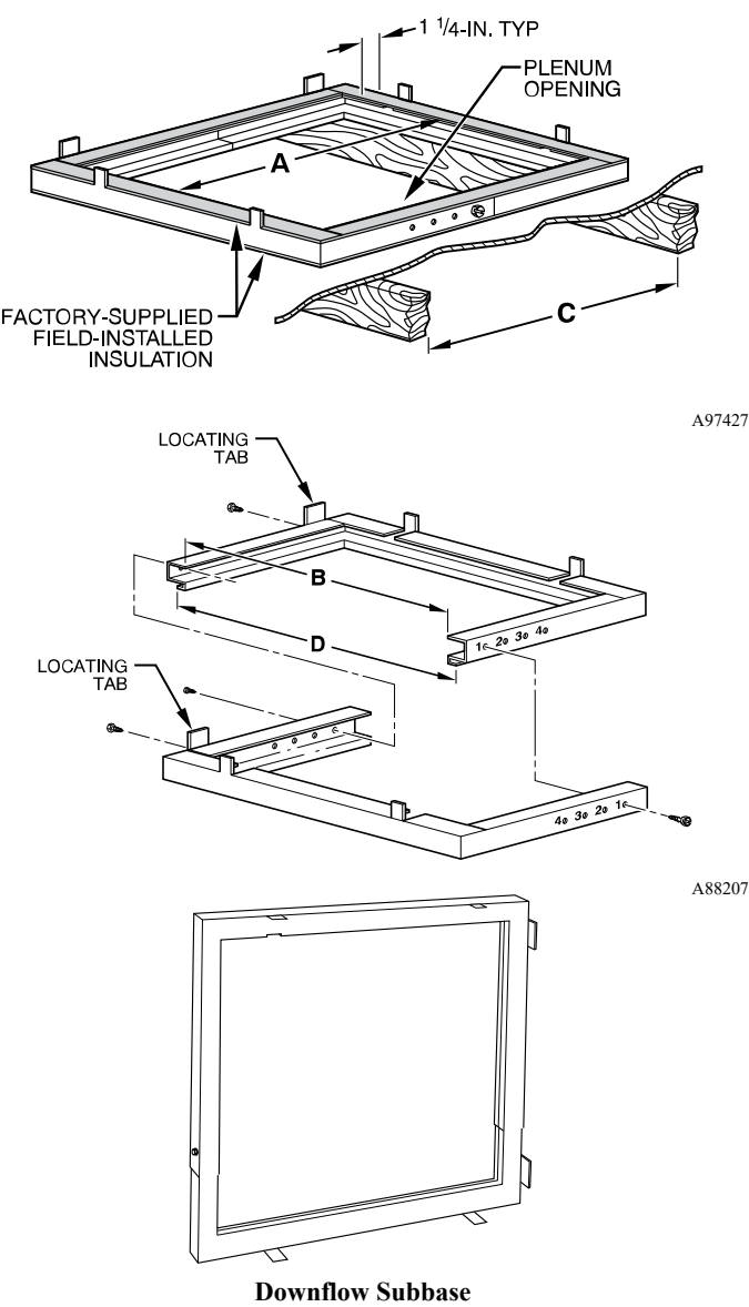
Downflow Subbase
