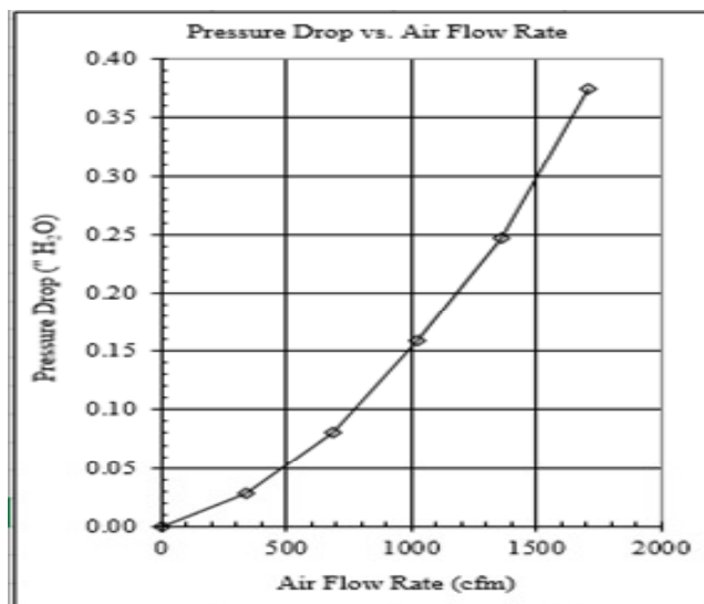
25" x 16" x 4" Filter (.20" @ 1,200 cfm) Pressure Drop Chart
