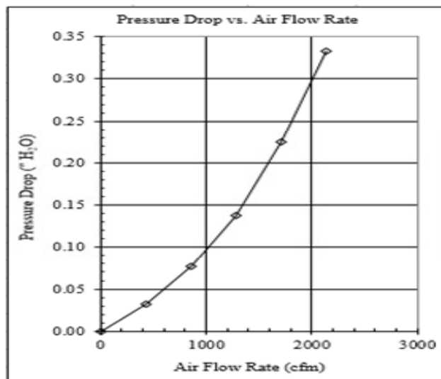
25" x 20" x 4" Filter (.20" @ 1,600 cfm) Pressure Drop Chart
