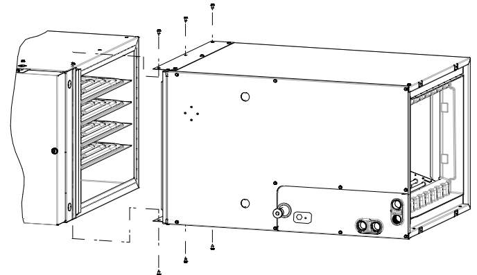
Fig. 6 – Horizontal-Right Installation
