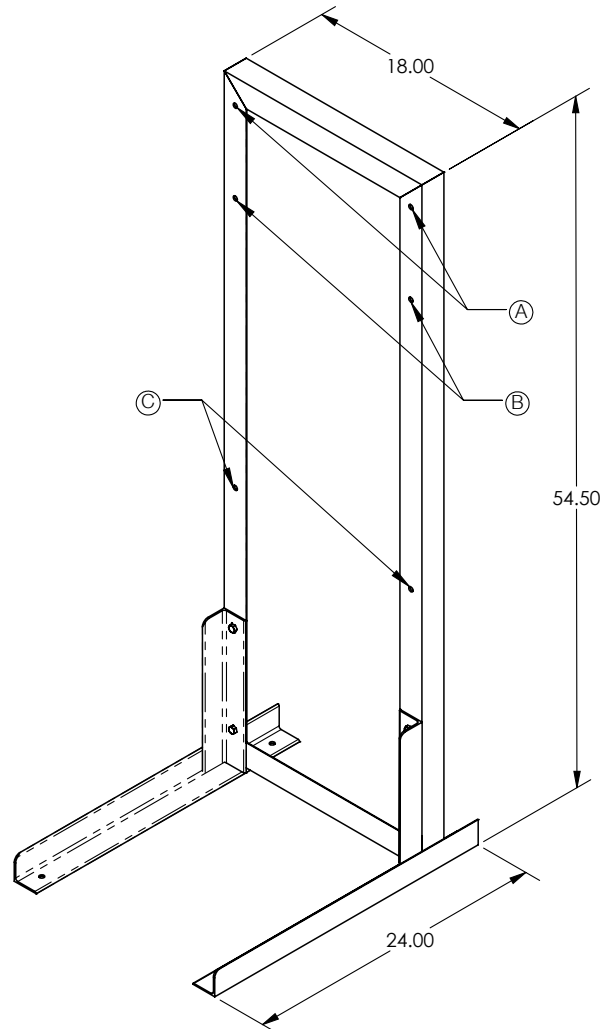
Figure 1: Floor Stand Assembly
