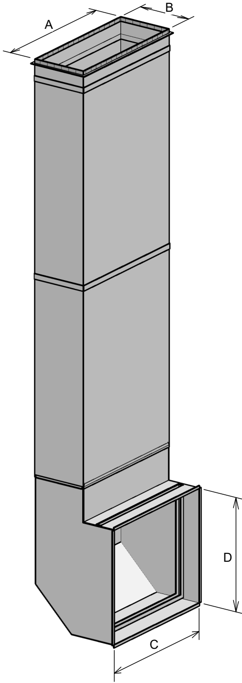
COLD AIR TOP LOAD DROP KIT
