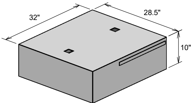
1" SHORT RETURN AIR BASE
