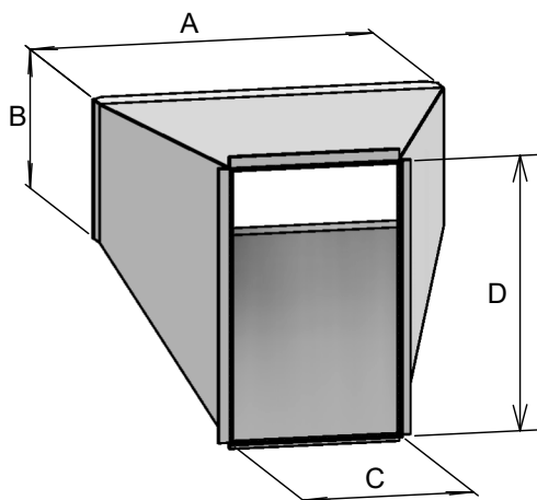
TRANSITION START COLLAR
