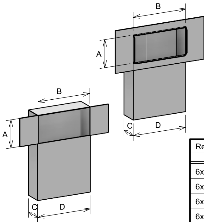
STACK HEAD
