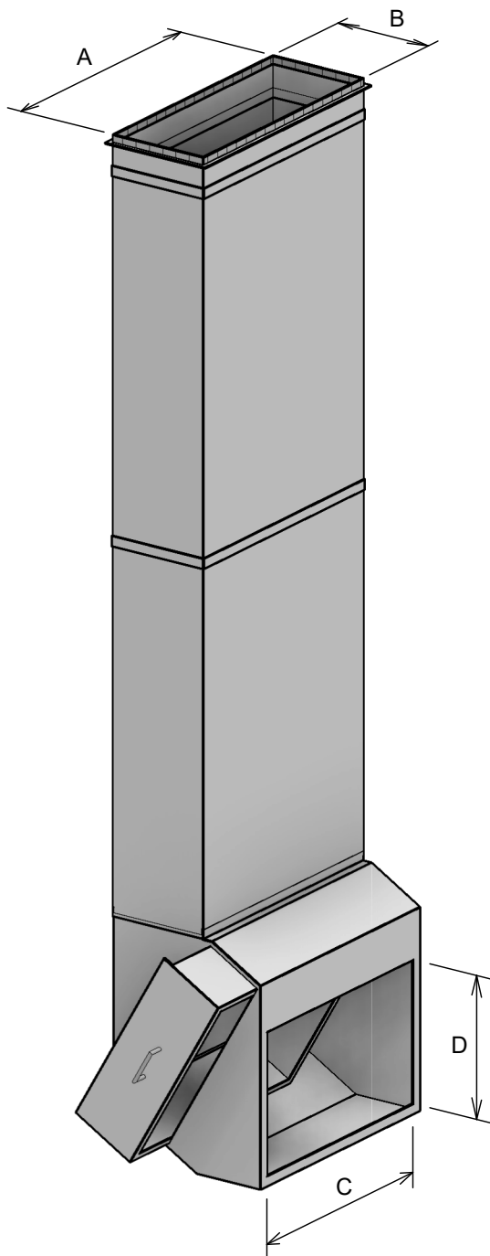
ALTERAIRE BOOT WITH DRAWER DROP KIT
