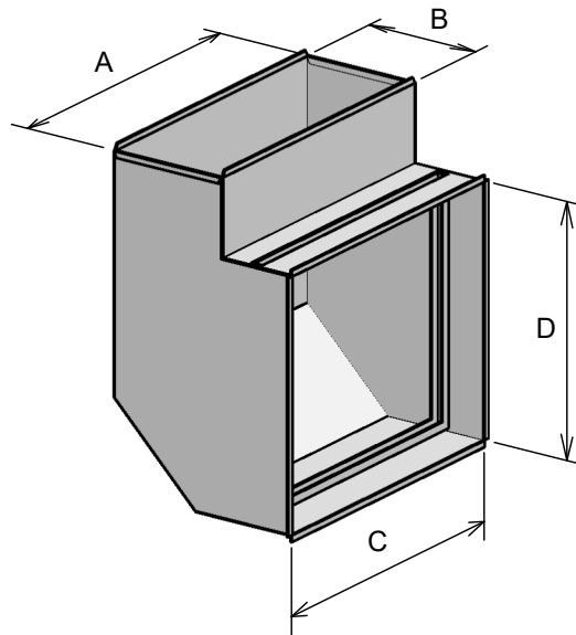
FILTER BOOT TOP LOAD
