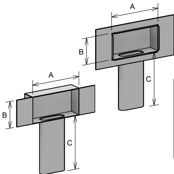
OVAL STACK HEAD
