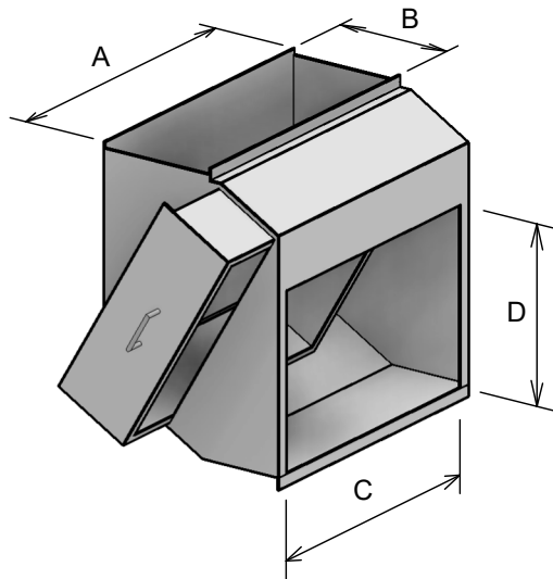
MODIFIED ALTERAIRE BOOT WITH DRAWER
