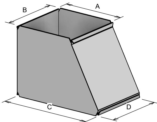
DUCT TRANSITIONS
