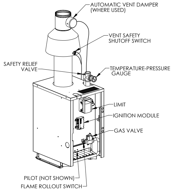
Figure 1: Control Locations
