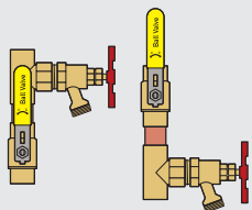
Draining from Above Ball Draining from Below Ball
