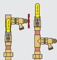
Draining from Above Ball Draining from Below Ball
