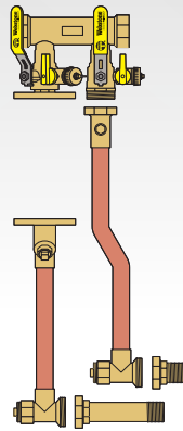
HYDRO-CORE™ COMPLETE NEAR BOILER PIPING KITS
