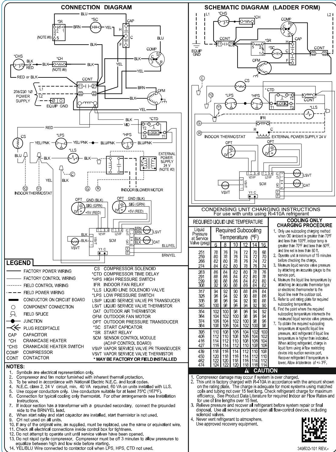
Fig. 1 – 127TBN024-60 Wiring Diagram
