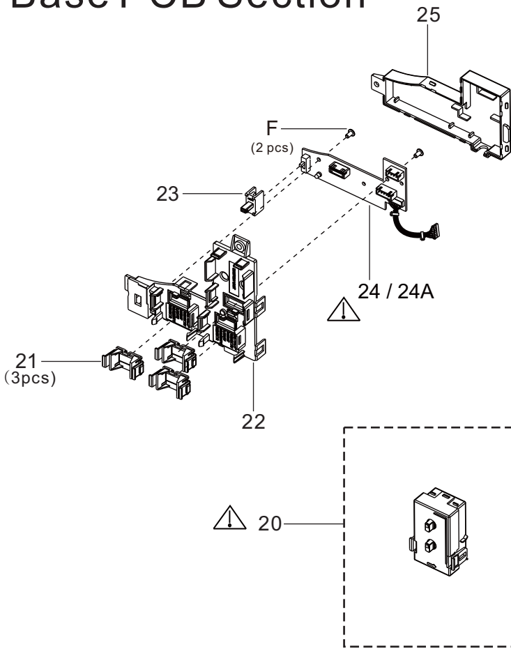
Multi-Speed Control Module
