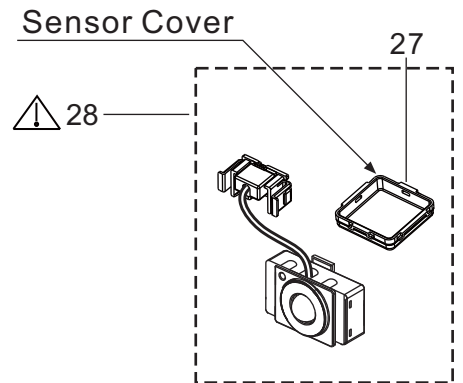
Motion Sensor Module
