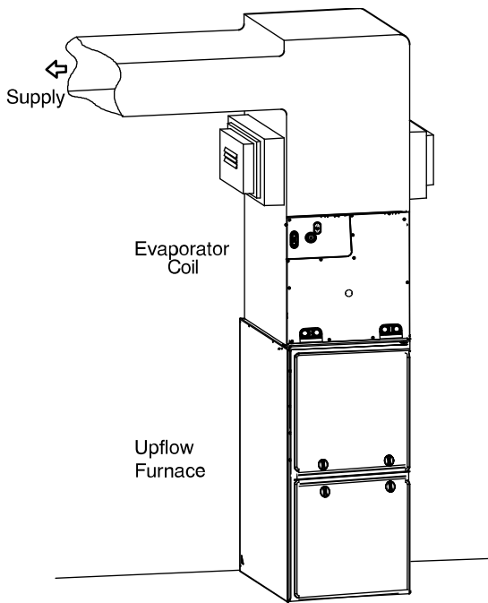
Fig. 16 – Humidifier Application
