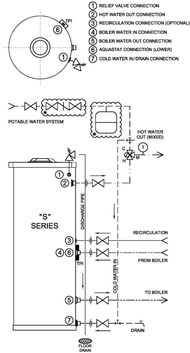
Figure 2-2 IWH Domestic Plumbing Schematic
