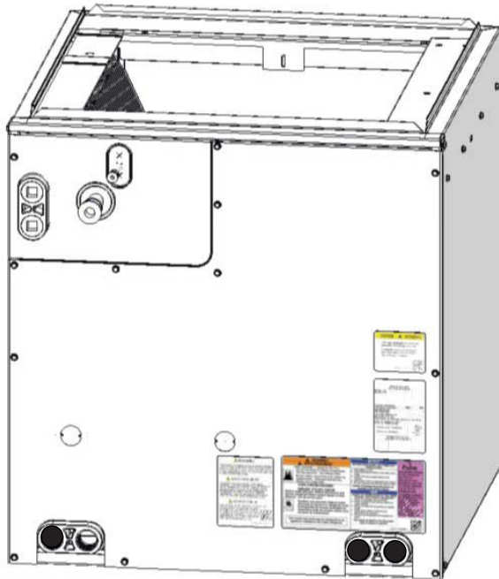
Fig. 1 – Typical Coil
