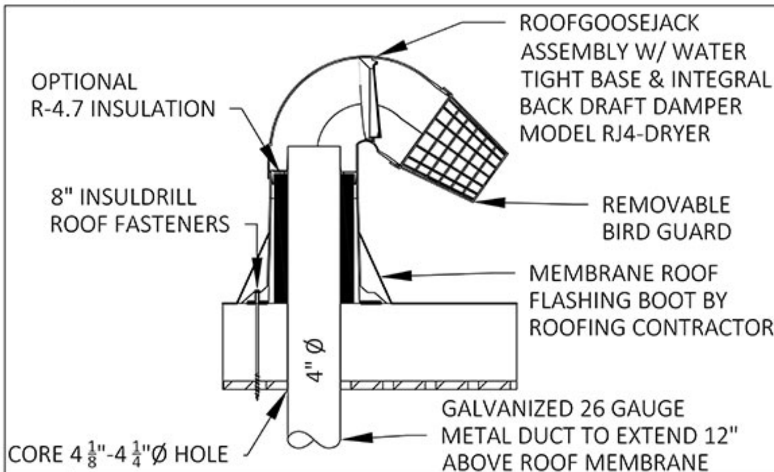
④ RJ4-DRYER TERMINATION INSTALL DETAIL NOT TO SCALE
