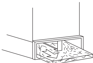
Fig. 16 – Slide Side Filter Out of Furnace
