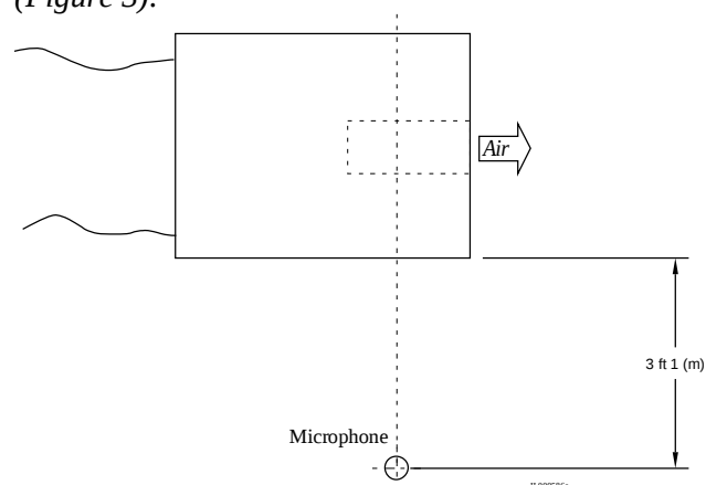
Figure 3. Location of Sound Level Meter
